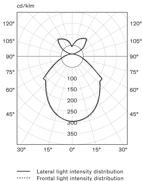
Example of light intensity distribution at 16 W
